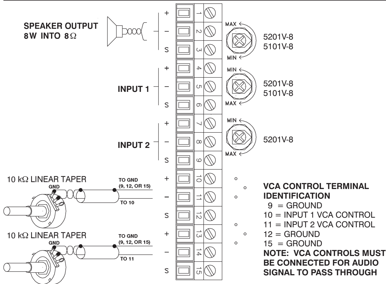
Figure 6 - 5032 Rear Panel Terminal Connections 5201V-8, 5251V-8, 5101V-8, 5151V-8
