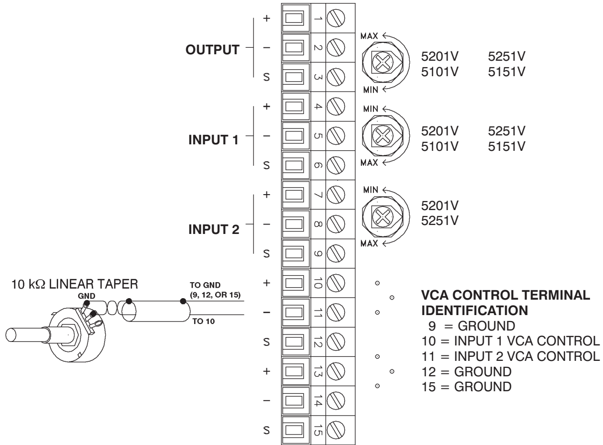
Figure 5 - 5032 Rear Panel Terminal Connections 5201V, 5251V, 5101V, 5151V
