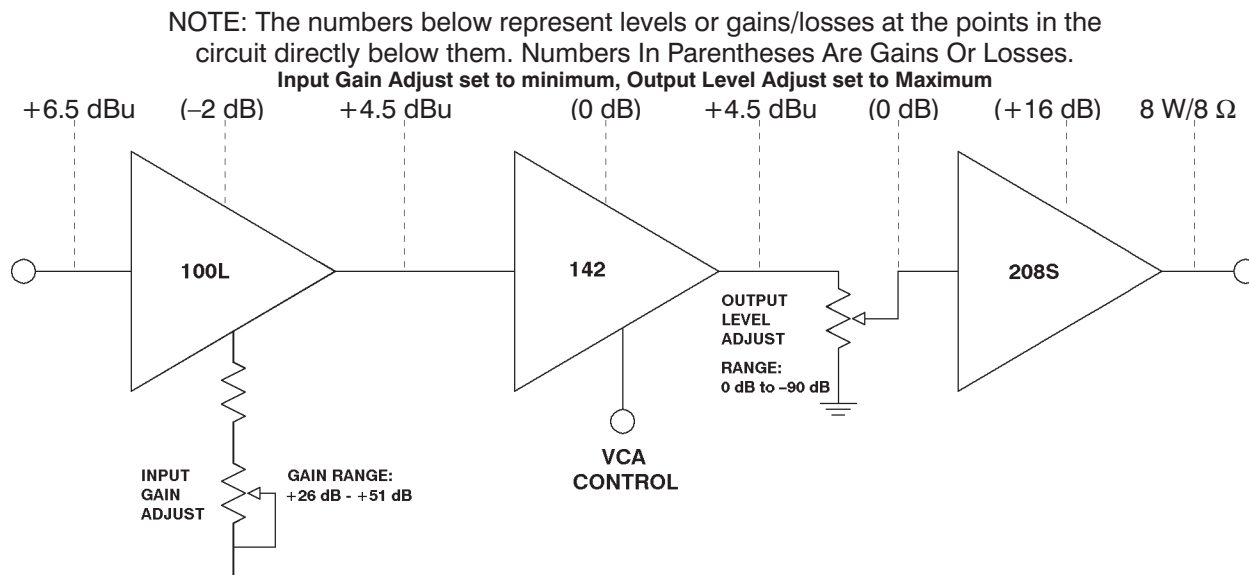
Figure 4 - Gain Structure 5101V-8, 5201V-8
