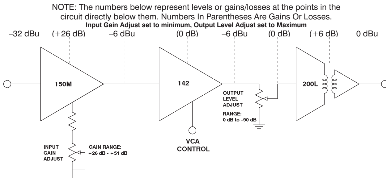
Figure 3 - Gain Structure 5151V, 5251V
