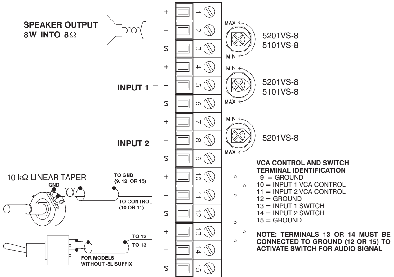
Figure 6 - 5032 Rear Panel Terminal Connections 5201VS-8, 5101VS-8
