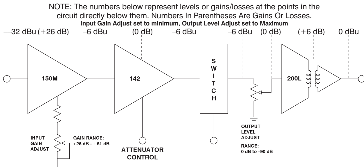
Figure 3 - Gain Structure 5151VS, 5251VS
