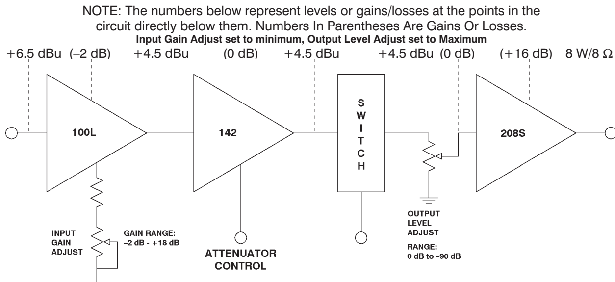
Figure 4 - Gain Structure 5101VS-8, 5201VS-8
