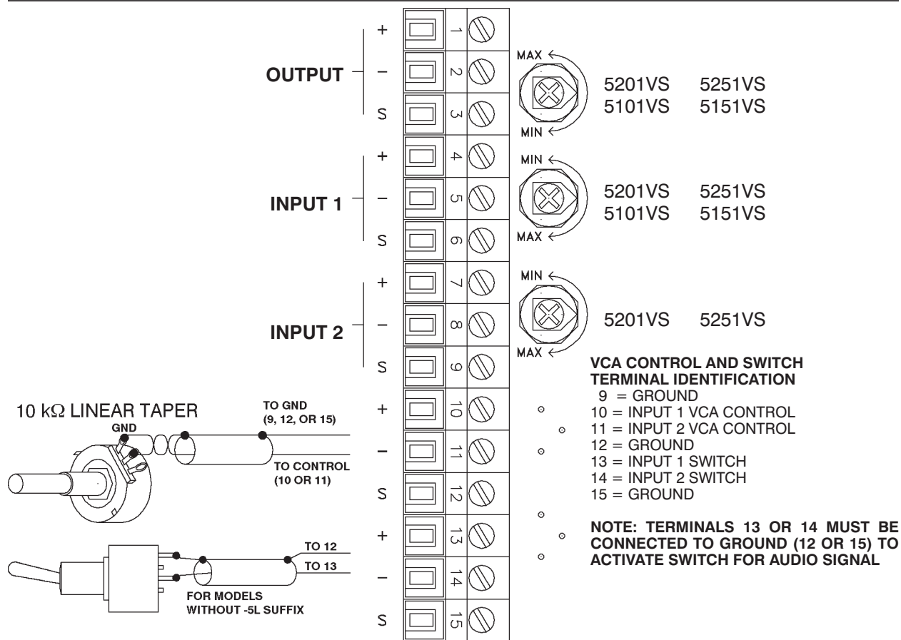
Figure 5 - 5032 Rear Panel Terminal Connections 5201VS, 5251VS, 5101VS, 5151VS
