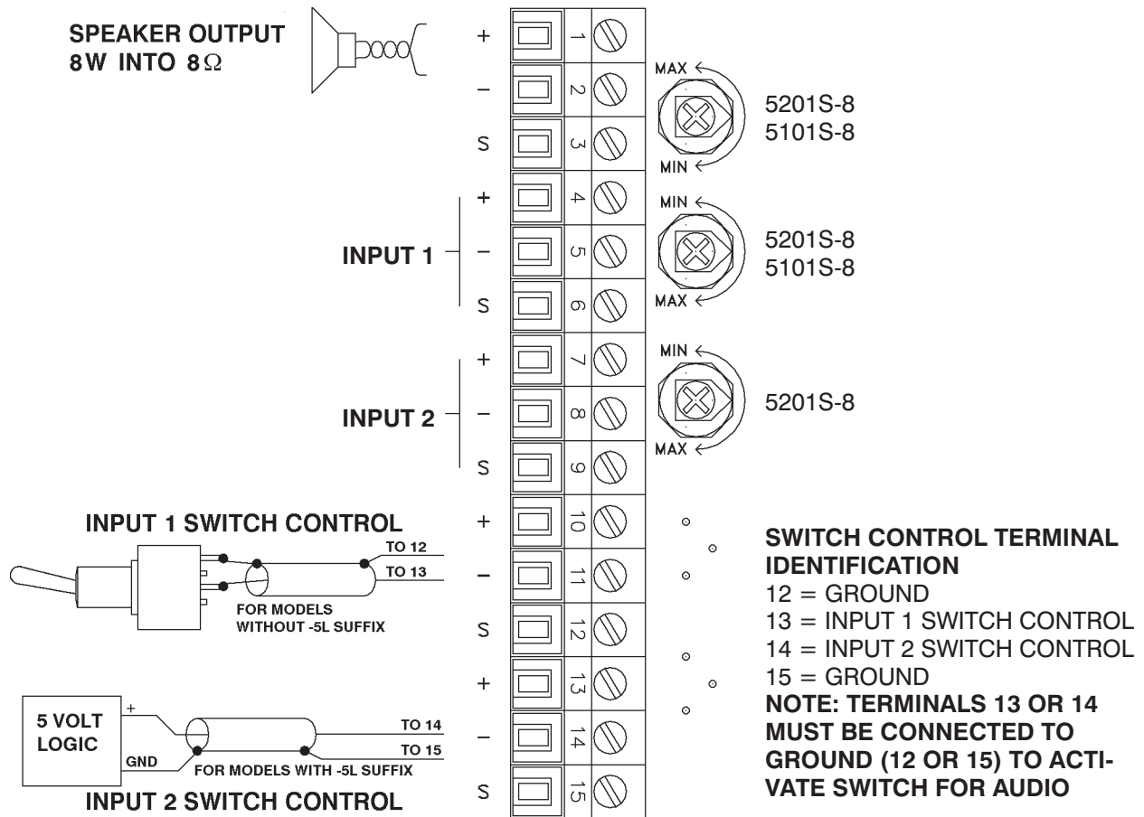
Figure 6 - 5032 Rear Panel Terminal Connections 5201S-8, 5101S-8
