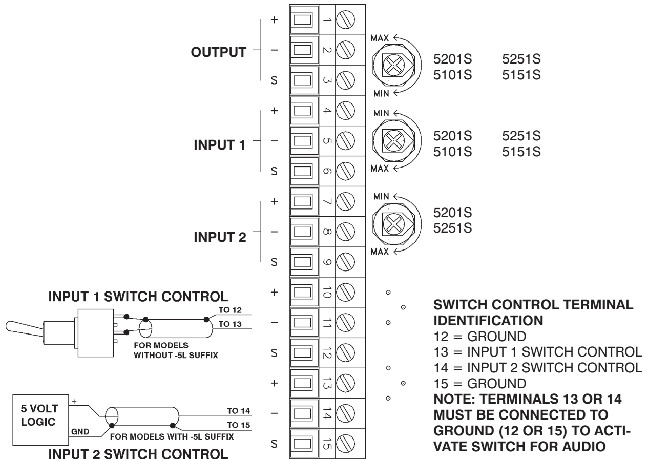
Figure 5 - 5032 Rear Panel Terminal Connections 5201S, 5251S, 5101S, 5151S
