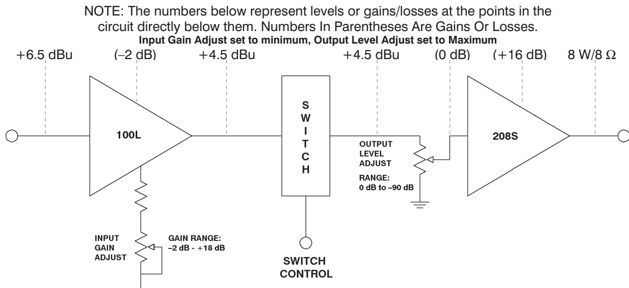
Figure 4 - Gain Structure 5101S-8, 5201S-8
