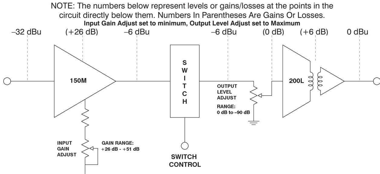
Figure 3 - Gain Structure 5151S, 5251S
