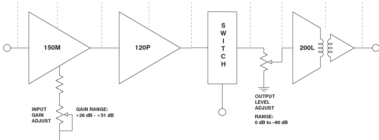
Figure 3 - Gain Setup Example 2 5251PS, 5151PS
