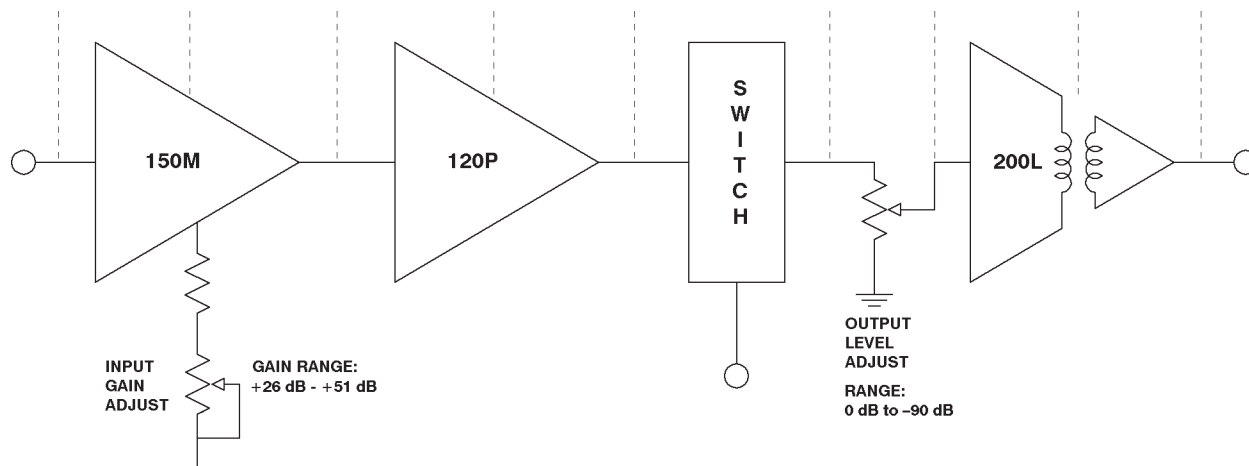
Figure 5 - Gain Structure 5251PS, 5151PS
