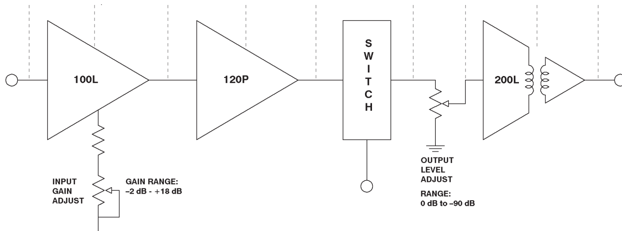
Figure 4 - Gain Structure 5101PS, 5201PS
