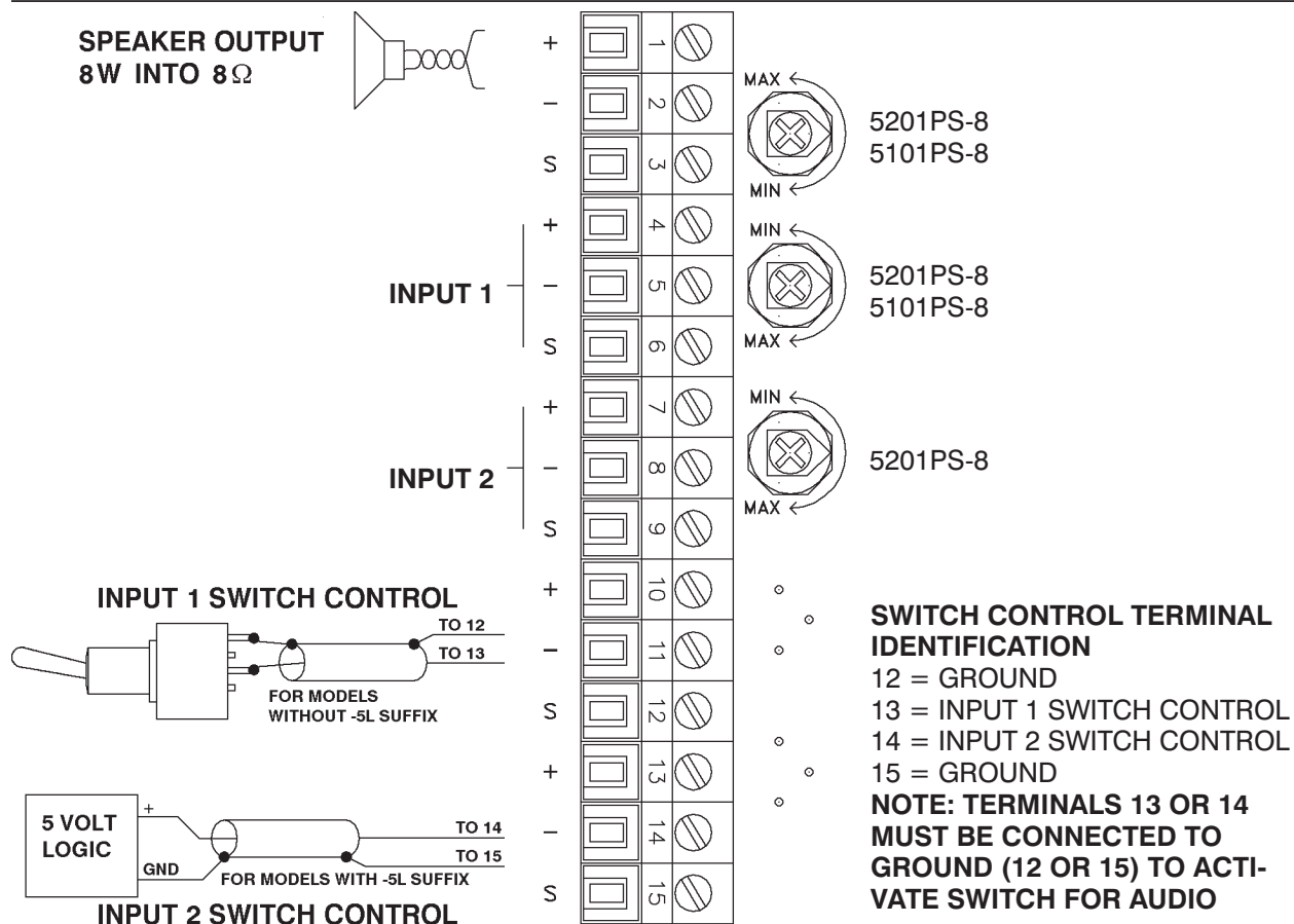
Figure 8 - 5032 Rear Panel Terminal Connections 5201PS-8, 5101PS-8
