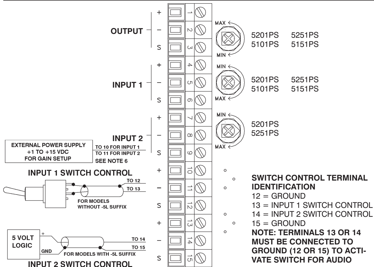
Figure 7 - 5032 Rear Panel Terminal Connections 5251PS, 5251PS, 5101PS, 5151PS
