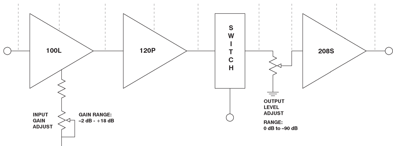
Figure 6 - Gain Structure 5101PS-8, 5201PS-8
