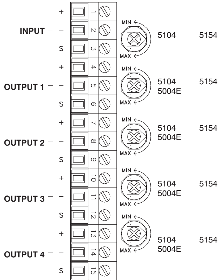
Figure 4 - 5032 Rear Panel Terminal Connections 5104, 5154, 5004E
