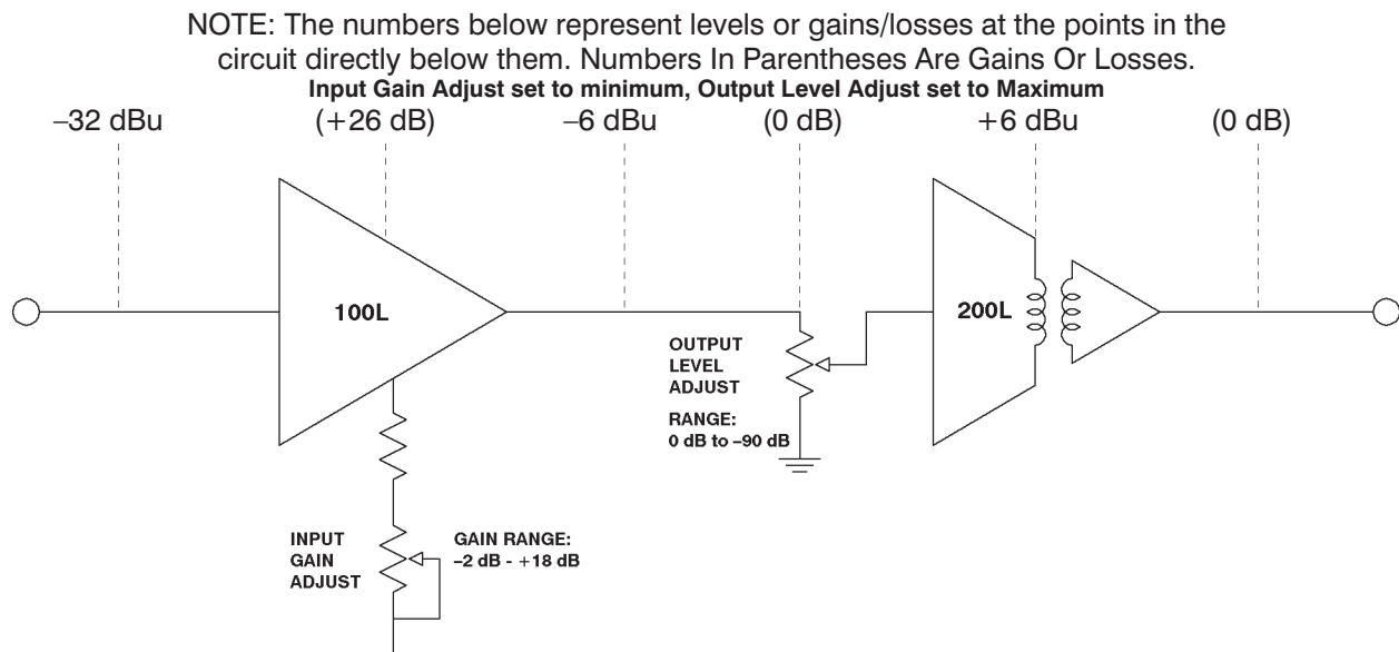
Figure 3 - Gain Structure 5154
