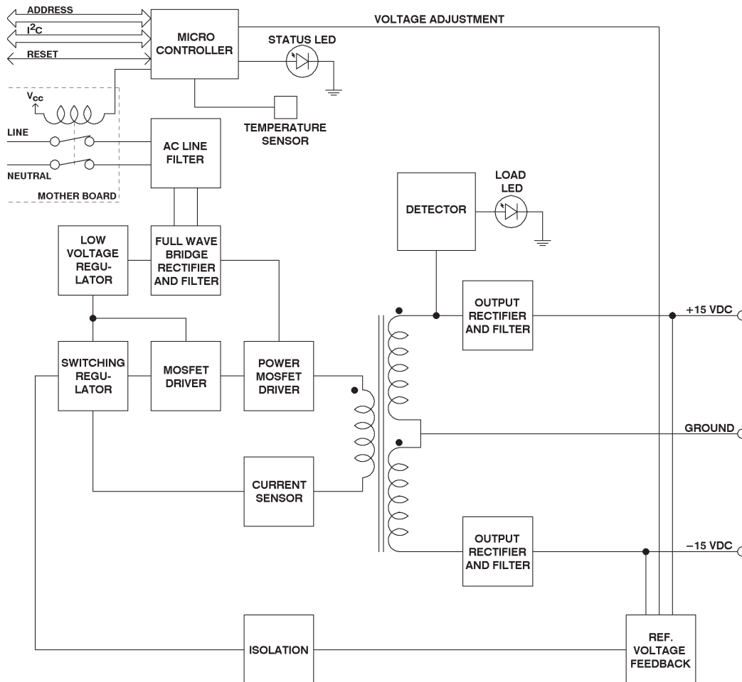
Figure 1 - 415L Power Supply Block Diagram
