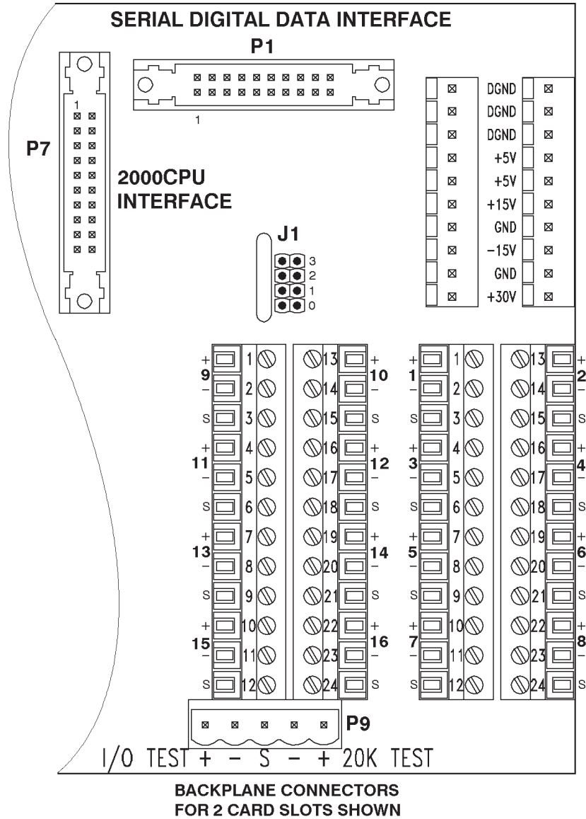
Figure 1 - 2008C Microphone Station Control Card 2012 Rear Panel Connections
