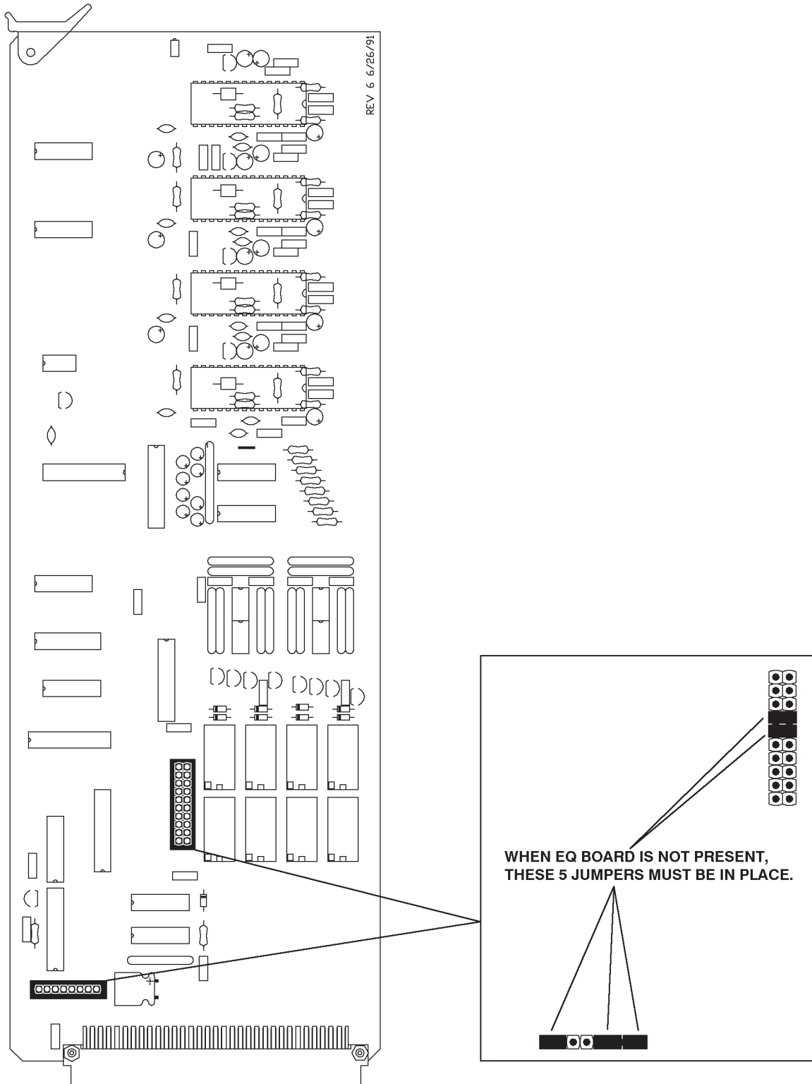
Figure 2 - Jumper placement when EQ card is not present
