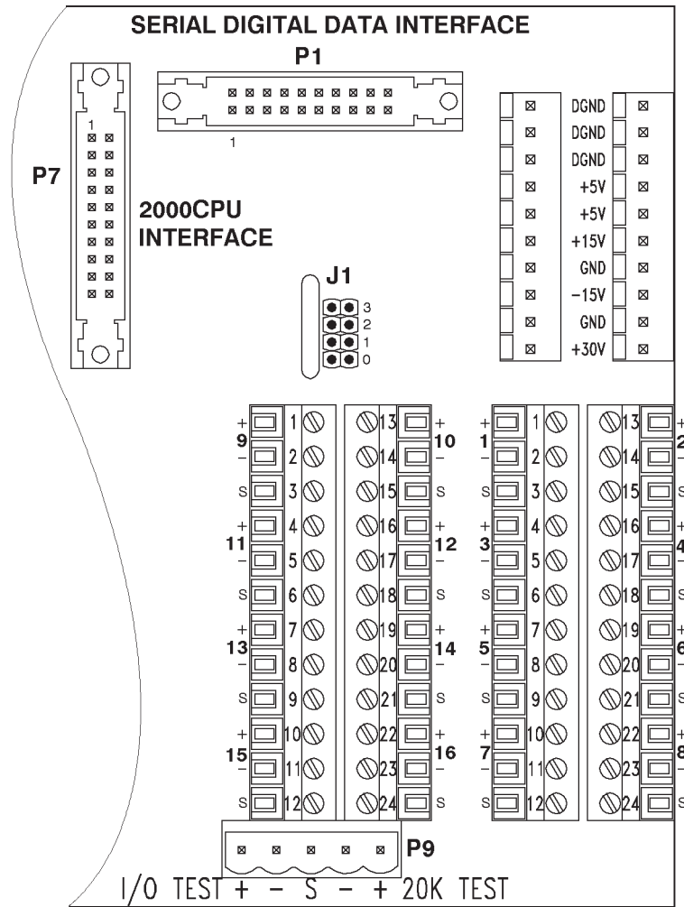
BACKPLANE CONNECTORS FOR 2 CARD SLOTS SHOWN
